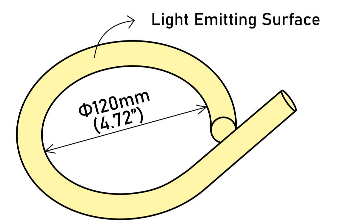
MINIMUM BENDING DIAMETER
