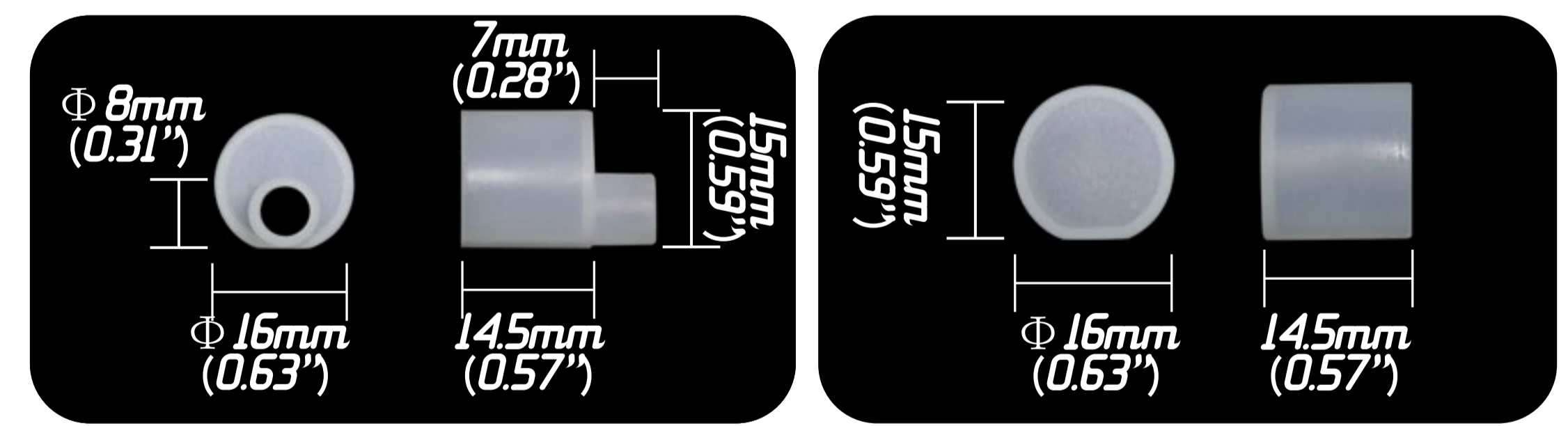
FRONT CONNECTION FITTING
