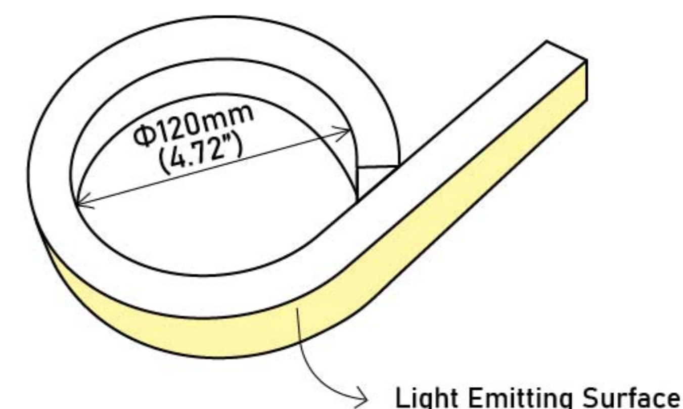
MINIMUM BENDING DIAMETER
